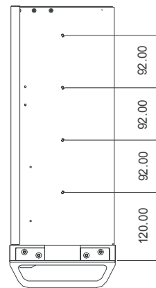
Right-side View
