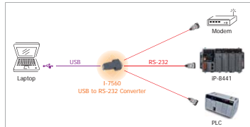
I-7560 with CA-USB18 I-7560 with IP-8441 I-7560 with Modem
